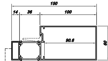
MUL0011830 ★ THK 1.5 0.430 kg/m MUL0013130 ★ THK 1.5 1.491 kg/m
