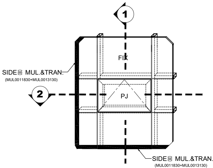
FIX & PROJECT ELEVATION (OUTSIDE VIEW)
