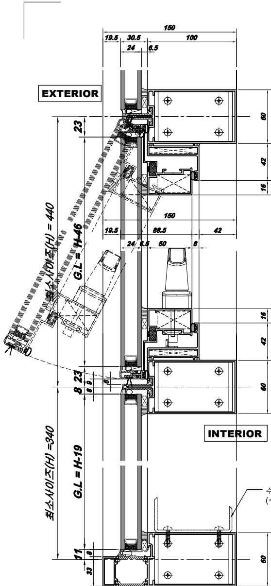
1 VERTICAL SECTION
