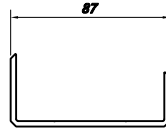
MUL0011245 ★ THK 3.0 1.179 kg/m (CW BRACKET)
