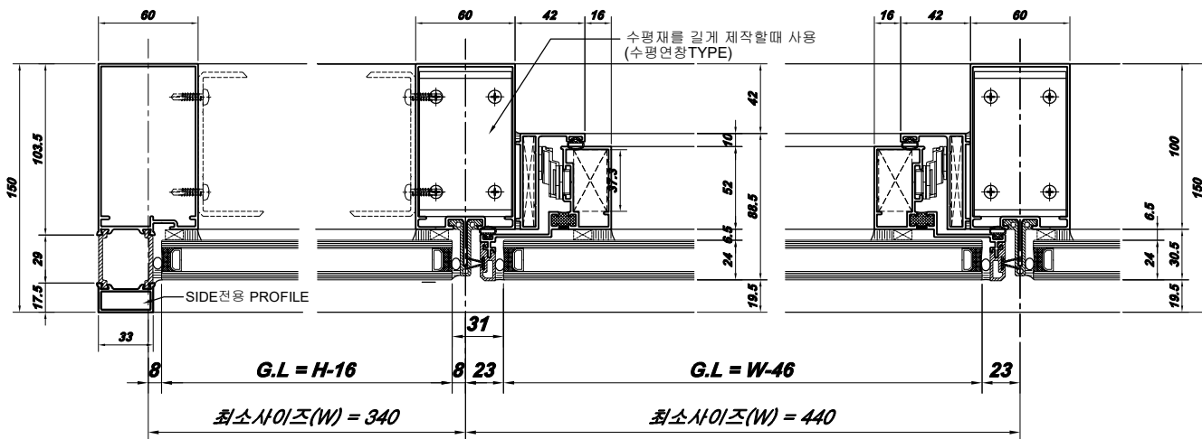
2 HORIZONTAL SECTION
