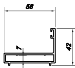
MUL0010636 ★ THK 1.6 0.769 kg/m
