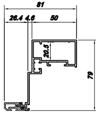
MUL0011828 ★ THK 1.6 1.179 kg/m
