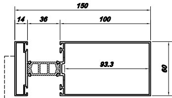
MUL0011789 ★ THK 1.7 0.705 kg/m MUL0012921 ★ THK 1.5 1.451 kg/m MUL0013237 THK 1.8 1.886 kg/m
