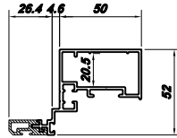
MUL0011827 ★ THK 1.6 1.062 kg/m
