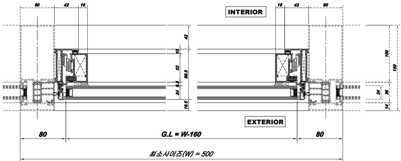
2 HORIZONTAL SECTION
