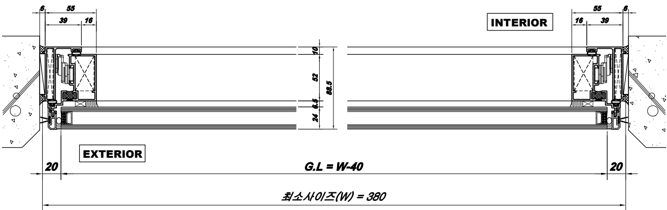
2 HORIZONTAL SECTION
