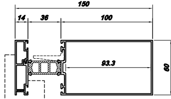
MUL0011790 ★ THK 1.4 0.465 kg/m MUL0011791 ★ THK 2.0 0.292 kg/m MUL0012921 ★ THK 1.5 1.451 kg/m MUL0013237 THK 1.8 1.886 kg/m
