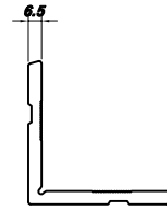
035PJ19115 ★ THK 6.5 2.263 kg/m
