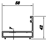
MUL0010636 ★ THK 1.6 0.769 kg/m
