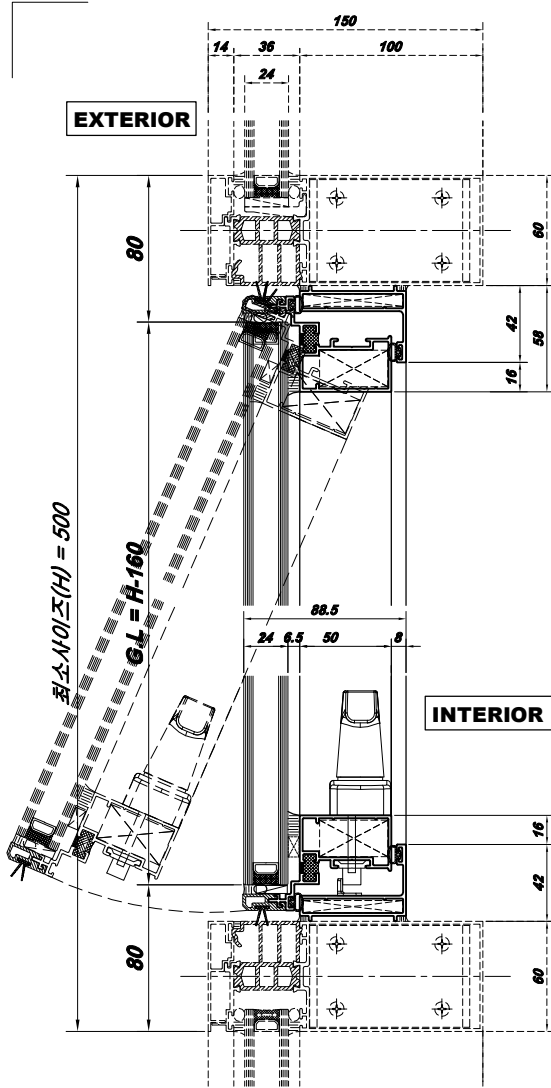
1 VERTICAL SECTION
