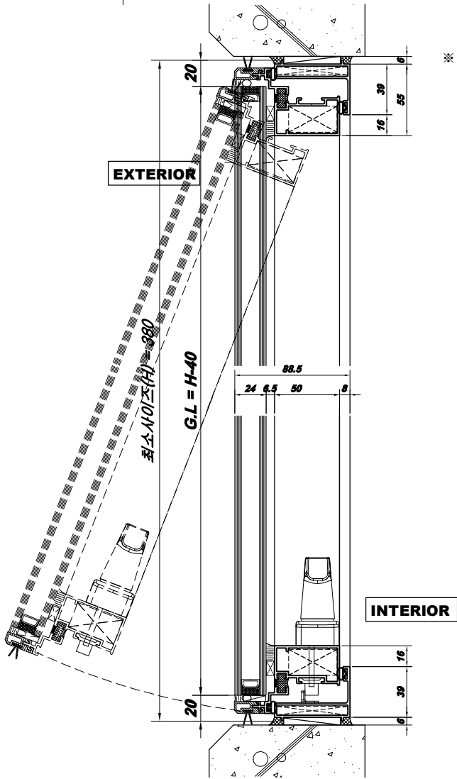
1 VERTICAL SECTION
