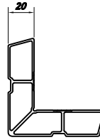
MUL0013016 THK 1.5 1.462 kg/m
